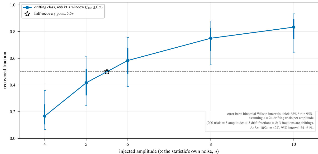
(b) fine 488 kHz configuration, drifting searched class
