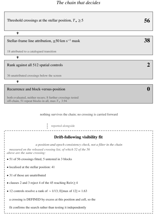
FIG. 7.— The chain that disposes of a threshold crossing, with the number surviving each step: 56 crossings, 18 identified as carbon monoxide by the stellar-frame line mask, 38 unattributed, 2 outranking every one of the 512 control positions, and none recurring in a later epoch. Every count is read from the ledger, so the figure and Table 5 cannot disagree. The visibility fit sits outside the column, because it is evaluated at the position and in the cell where the search already found an excess (§5.5.1).
