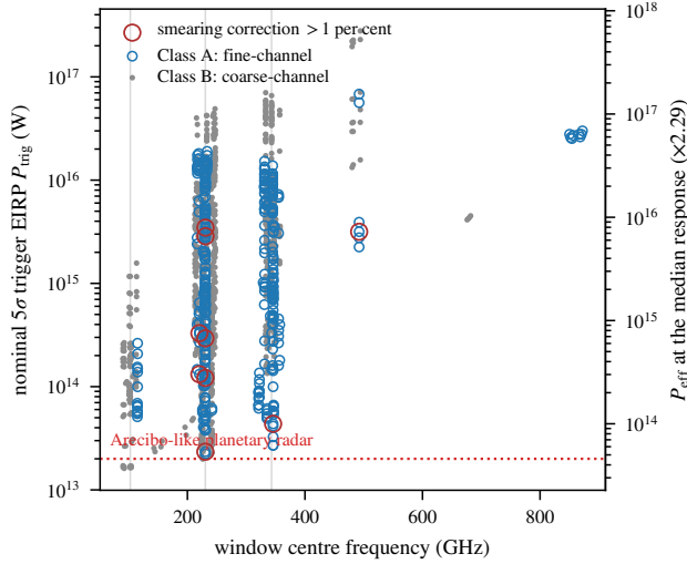
FIG. 9.— Two-dimensional sensitivity against window centre frequency for all 1655 searched windows, symbol by channelisation class, the axis along which completeness differs (Table 5). Left axis : the nominal trigger threshold P_{\text{trig}} , an internal detection statistic. Right axis : the effective threshold at the median response, P_{\text{eff}} = 2.29 P_{\text{trig}} , which is the power to compare with a transmitter (§4); the released per-window ratio P_{\text{eff, total}}/P_{\text{trig}} runs 1.33–3.98, so read a single window’s threshold from the catalogue and not from this axis. Red rings mark the 9 windows whose intra-integration smearing correction exceeds 1 per cent. Grey lines mark the Bands 3, 6 and 7 concentrations; dotted, the Arecibo 2.38-GHz EIRP benchmark, a power scale only. Note the two decades of scatter at fixed frequency: there is no single survey sensitivity.
