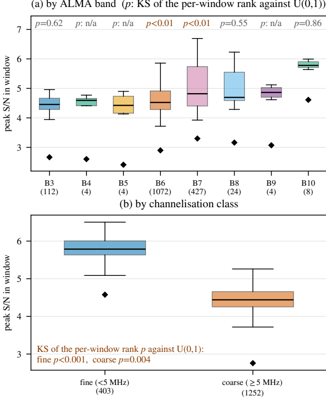
FIG. 12. — Exchangeability of the 512-position control ensemble by stratum, over 1655 windows. Boxes give the per-window control maximum, black diamonds the median on-star peak, and p the Kolmogorov–Smirnov test of the per-window rank against U(0,1) . (a) by ALMA band, with the window count under each label; (b) by channelisation class, fine (< 5 MHz) against coarse. The ensemble tracks the on-star statistic in every band, but both channelisation classes depart from uniformity: fine D = 0.150 , p < 10^{-4} over 403 windows, and coarse D = 0.050 , p = 0.004 over 1252. The departure is not the flagged windows’ doing — removing all 71 fine crossings leaves p = 0.002 — and §5.3.6 identifies the radial noise gradient as the cause.
