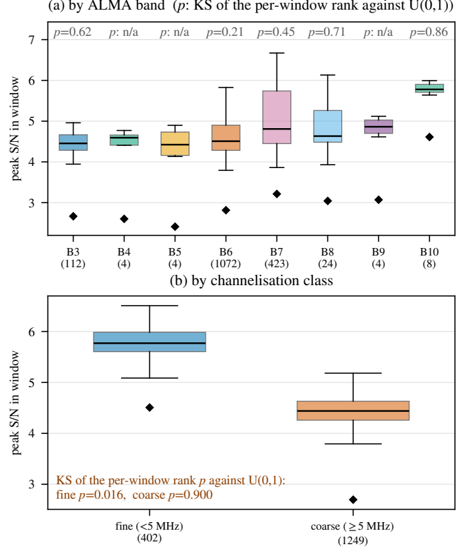
FIG. 13.— Exchangeability of the 512-position control ensemble by stratum, over 1651 windows. Boxes give the per-window control maximum, black diamonds the median on-star peak, and p the Kolmogorov–Smirnov test of the per-window rank against U(0, 1) . (a) by ALMA band, with the window count under each label; (b) by channelisation class, fine (< 5 MHz) against coarse. The ensemble tracks the on-star statistic in every band, and the fine class sits higher than the coarse, 5.77 against 4.44, as its larger trial count predicts. The fine class departs from uniformity, D = 0.077 ( p = 0.016 ); the coarse class does not, D = 0.016 ( p = 0.900 ). The departure is not the flagged windows’ doing — removing all 52 fine crossings lowers the statistic only to 0.086 — and §C.1.2 identifies the radial noise gradient as the cause.
