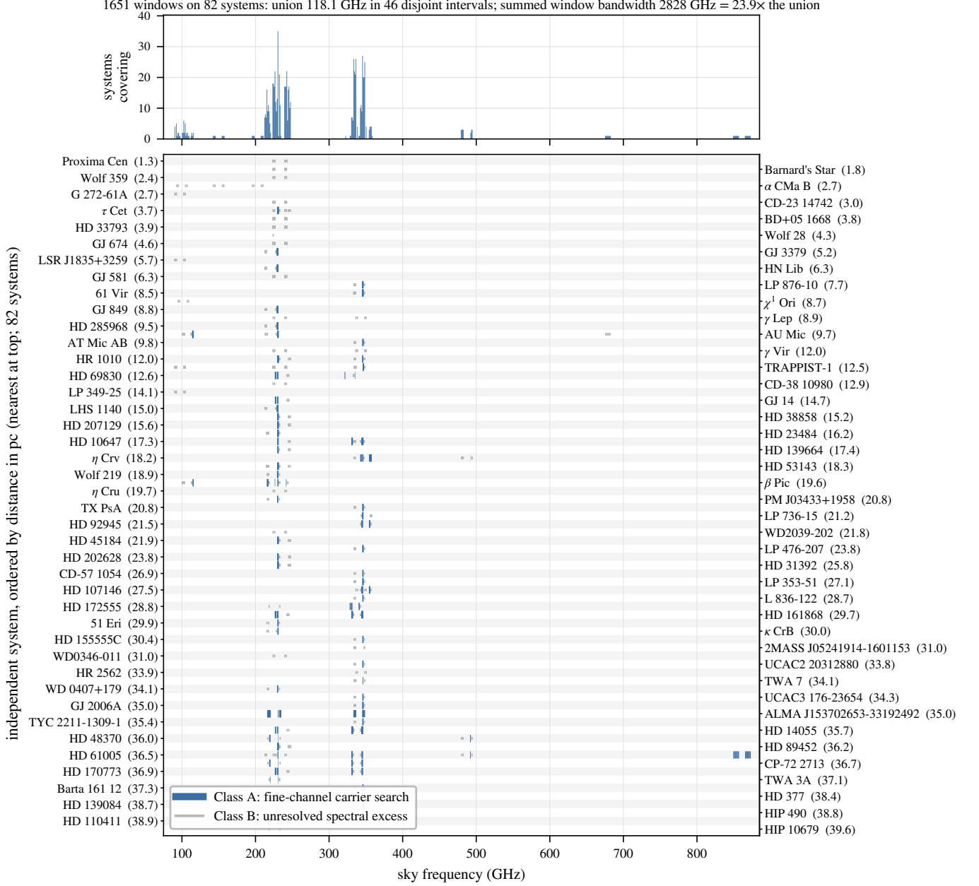
FIG. 7.— Where this survey searched. Lower panel: each searched window is a horizontal segment on its host system’s row, rows ordered by distance and labelled alternately on the left and right axes; heavy blue marks the fine-channel carrier search (Class A) and light grey the coarse-channel spectral-excess search (Class B). Upper panel: the number of systems covering each gigahertz of sky frequency; the threshold distribution is Fig. 1. The coverage is narrow, clustered and repeatedly revisited: 46 islands concentrated near 230 and 345 GHz, with summed window bandwidth 23.9 \times the union. The union measures frequency coverage, the summed bandwidth integrated search effort.
