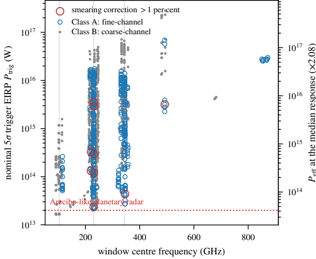
FIG. 9.— Two-dimensional sensitivity against window centre frequency for all 1651 searched windows, symbol by channelisation class, the axis along which completeness differs (Table 15). Left axis: the nominal trigger threshold P_{\text{trig}} , an internal detection statistic. Right axis: the effective threshold at the median response, P_{\text{eff}} = 2.08 P_{\text{trig}} , which is the power to compare with a transmitter (§4); the per-window ratio P_{\text{eff, total}}/P_{\text{trig}} runs 1.06–3.63, so a single window’s threshold should be read from the catalogue, not from this axis. Red rings mark the 9 windows whose smearing correction exceeds 1 per cent; dotted, the Arecibo 2.38-GHz benchmark. Note the two decades of scatter at fixed frequency: there is no single survey sensitivity.
