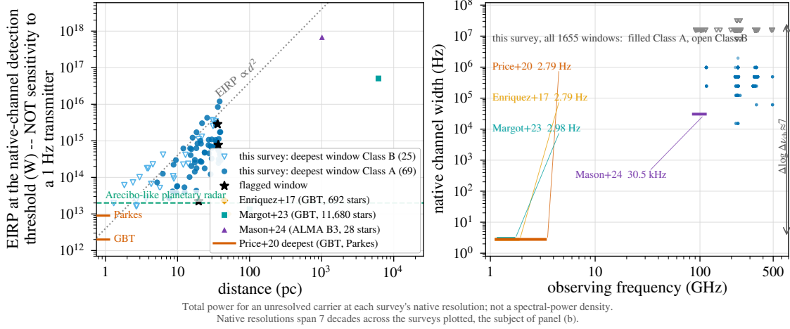
FIG. 1.— Literature context of the 5σ trigger thresholds, in total power (§2). (a) EIRP against distance. Blue: this survey, deepest window per star (94 stars, 1.30–39.63 pc; filled: Class A, fine-channel; open: Class B, coarse-channel); orange: Enriquez et al. (2017); aqua: Margot et al. (2023); violet: Mason et al. (2024); left-edge ticks: deepest per-target limits of Price et al. (2020). Grey dotted: EIRP ∝ d 2 at constant received flux. Green dashed: the Arecibo 2.38-GHz EIRP benchmark, a power scale only (§4.3). (b) Native channel width against observing frequency for the same windows and programmes: resolutions differ by ∼10 7 , so the panels must be read together and a lower EIRP here does not imply greater sensitivity to a hertz-wide carrier. This is not a like-for-like sensitivity comparison. The 5σ plotted for each programme is that programme’s own threshold statistic, and those statistics differ in definition, in the channel width they are evaluated over and in the completeness they correspond to; for this survey it is a trigger power with 42–61 per cent recovery, not a detection limit (Table 1). Our plotted values also exclude the ×2.29 median spectral-response correction and the ×1.41 available from the individual parallel hands, so a transmitter comparison carries a further ×3.2 against this survey’s curve at the median response, more in the tail.
