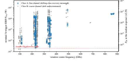
FIG. 7.— Two-dimensional sensitivity against window centre frequency for all 1655 searched windows, symbol by channelisation class, the axis along which completeness differs (Table 5). Left axis : the nominal trigger threshold P_{\text{trig}} , an internal detection statistic. Right axis : the effective threshold at the median response, P_{\text{eff}} = 2.29 P_{\text{trig}} , which is the power to compare with a transmitter (§4); the released per-window ratio P_{\text{eff, total}}/P_{\text{trig}} runs 1.33–3.98, so read a single window’s threshold from the catalogue and not from this axis. Ringed symbols are the 9 windows whose intra-integration smearing correction exceeds 1 per cent. Grey lines mark the Bands 3, 6 and 7 concentrations; dotted, the Arecibo 2.38-GHz EIRP benchmark, a power scale only. Note the two decades of scatter at fixed frequency: there is no single survey sensitivity.
