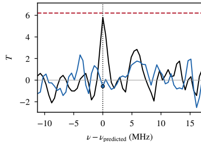
(f) CP-72 2713, and its repeat 2.0 h later
