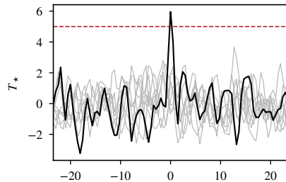
(f) CP-72 2713, and its repeat 2.0 h later
