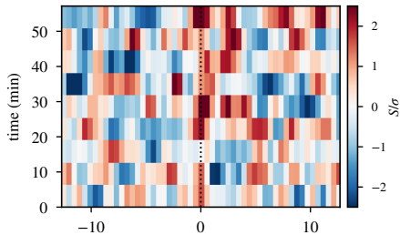
(e) 61 Vir, 3 repeats combined
