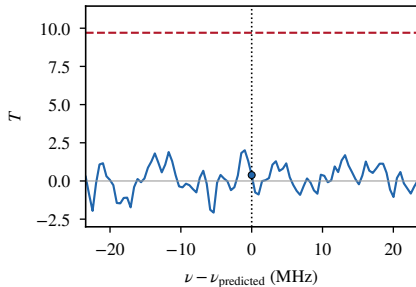
(e) 61 Vir, 3 repeats combined
