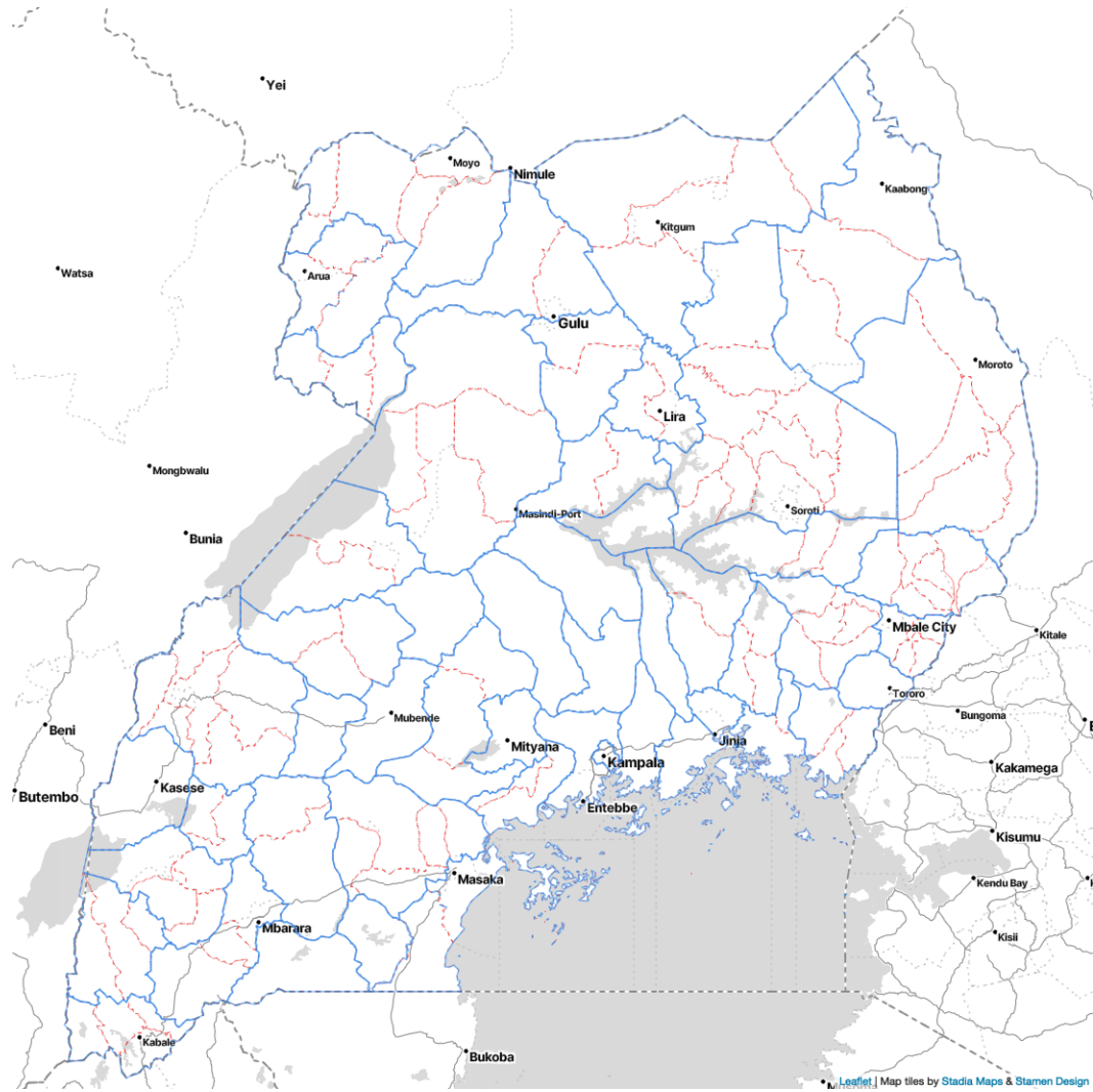
Figure A.14: Model geography.
