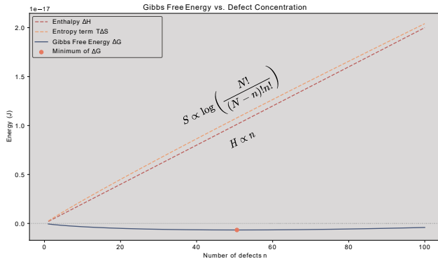
Figure 1. Gibbs free energy as a function of defect concentration. The minimum of the curve represents the state of equilibrium, where the system has a nonzero amount of defects in the crystal lattice. The increase in Gibbs free energy is due to the increase in enthalpy, while the decrease in Gibbs free energy is due to the increase in entropy.
