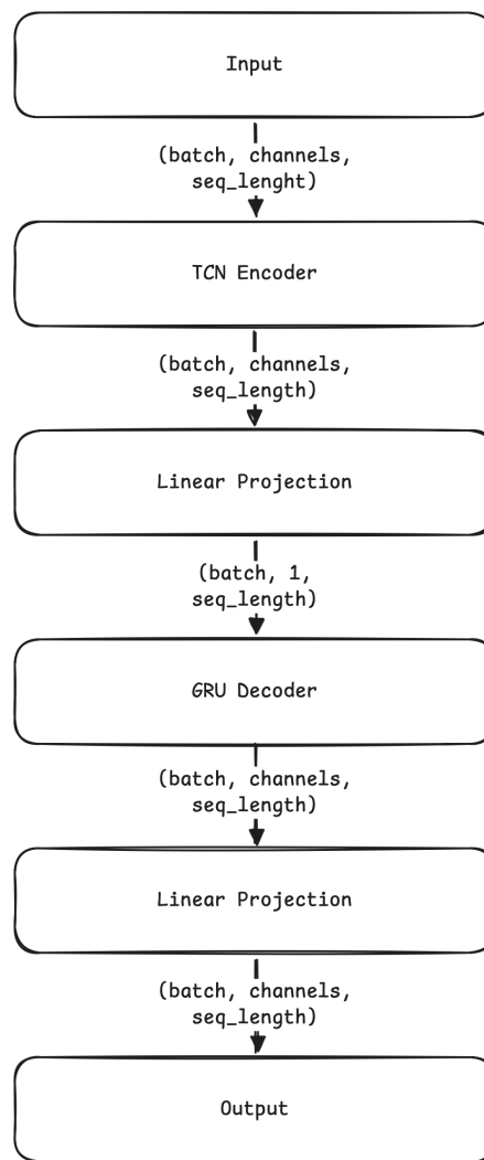
Figure 3.1: TCN-RNN architecture
