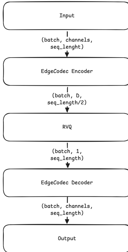
Figure 3.3: EdgeCodec architecture
