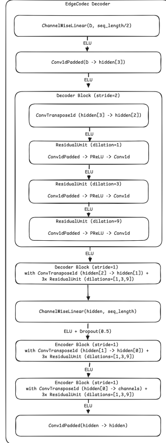
Figure 3.5: EdgeCodec decoder
