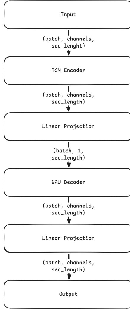
Figure 4.3: TCN-RNN Architecture
