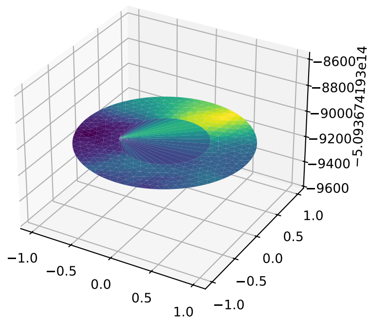
Numerical solution ( N = 352 , m = 608 )
