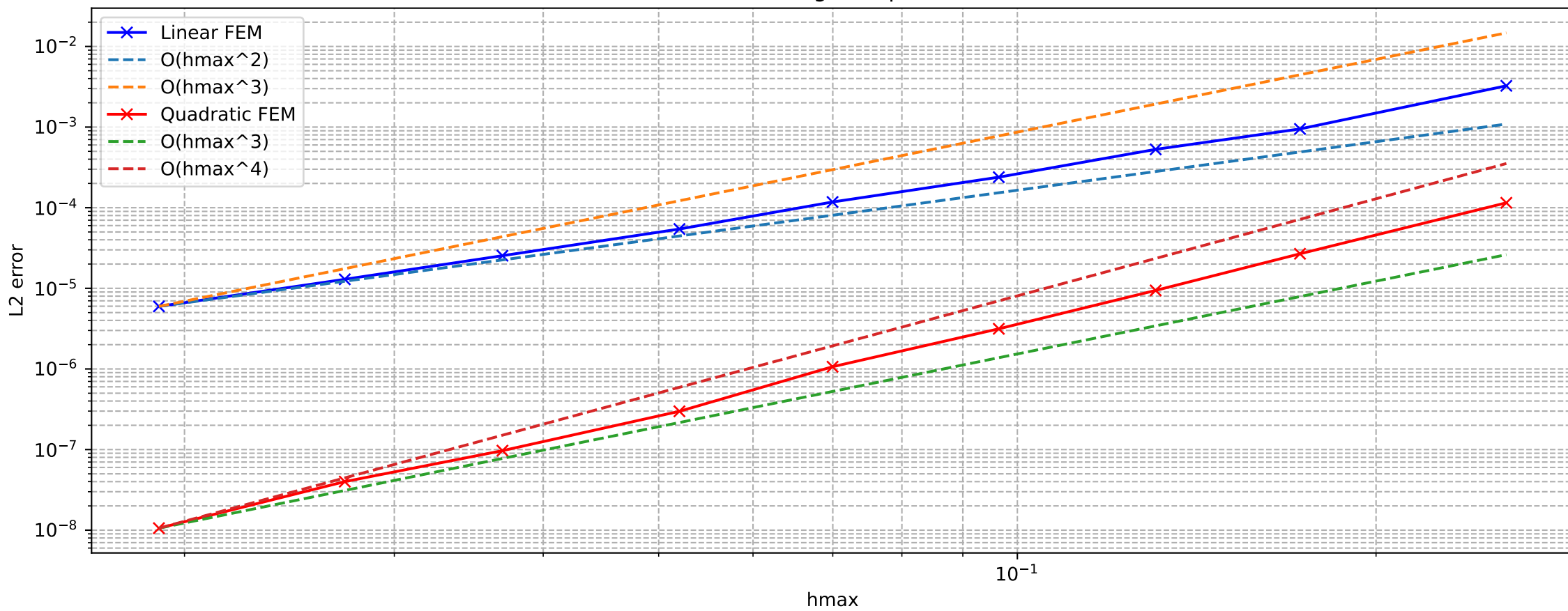
Work-Precision
