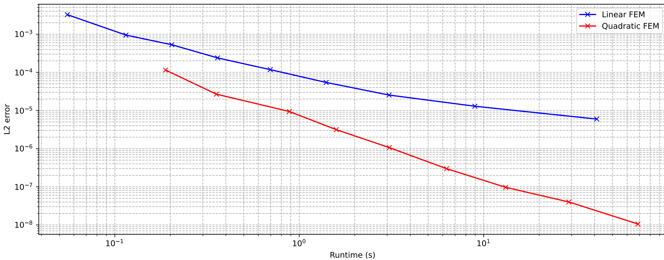
Work-Precision
