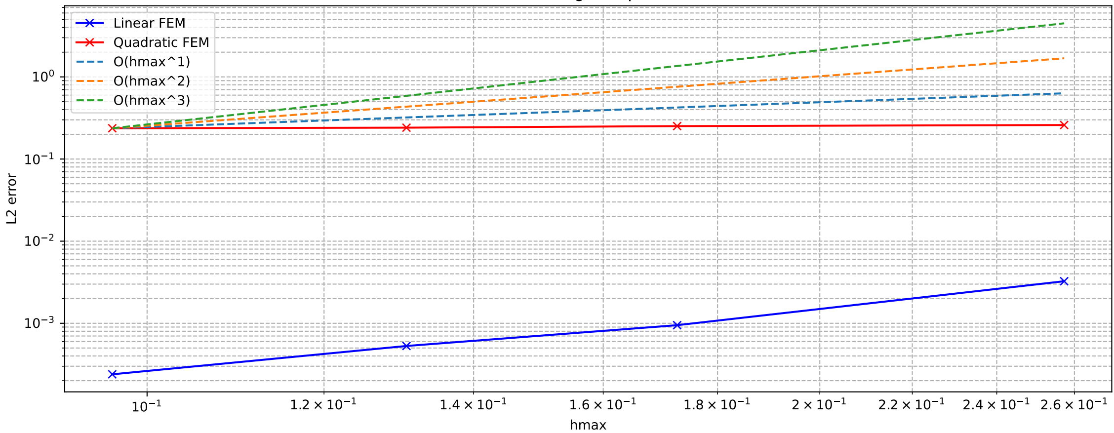
Work-Precision
