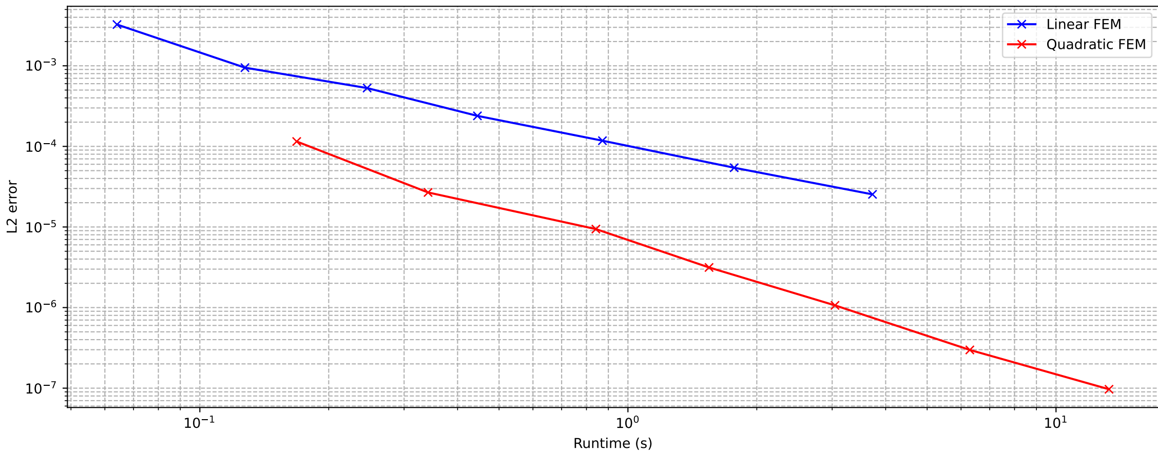
Work-Precision
