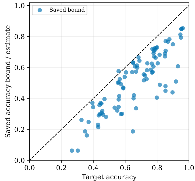
DIS2 historical
