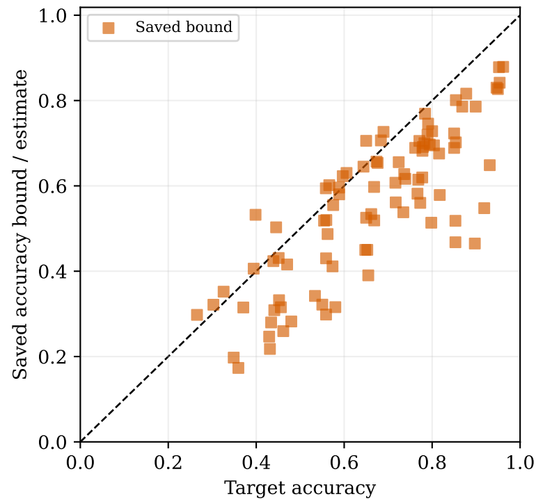
DIS2 reference
