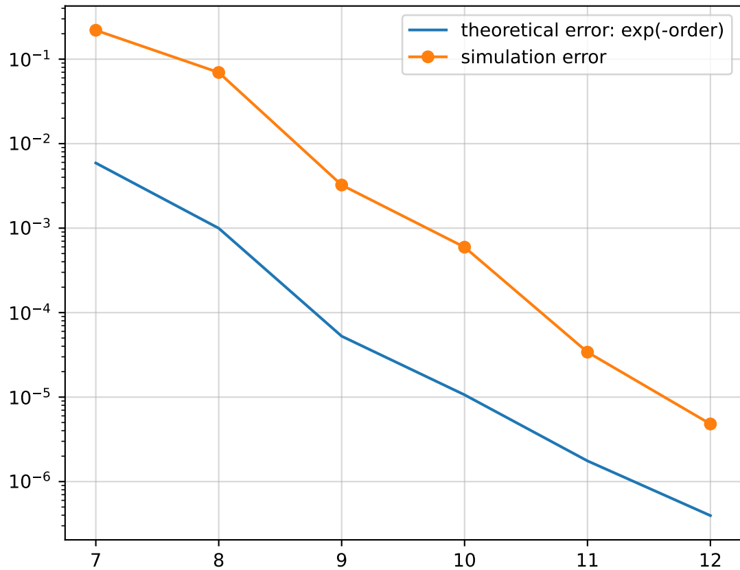
CQ Error vs Interpolation Order
