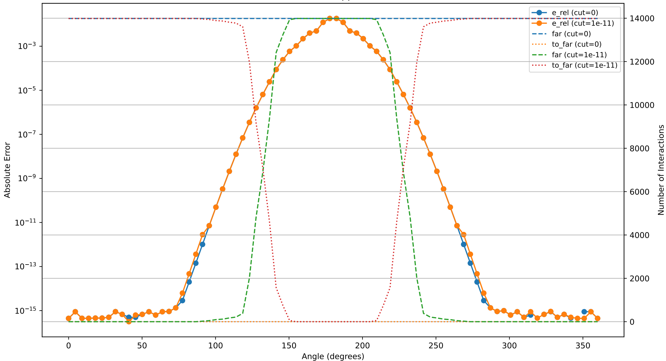
Relative Error + Interaction Counts over CQ circle of complex wavenumbers Shifted circle (kappa = 100.0)
