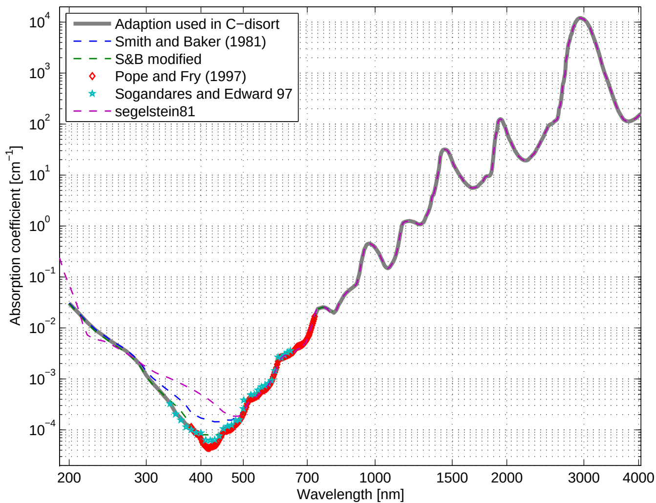
Measured absorption coefficient of pure water
