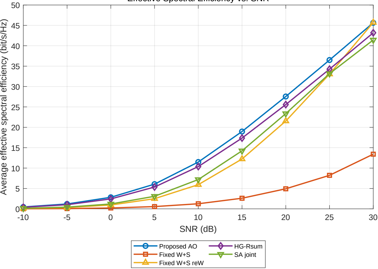
Effective Spectral Efficiency vs. SNR
