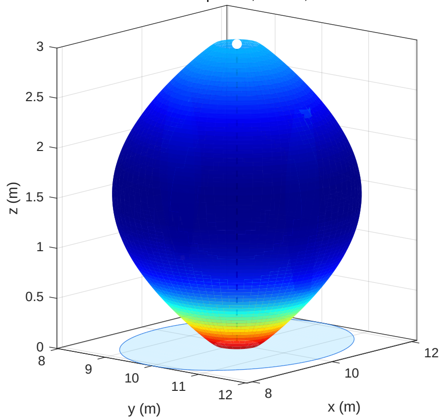
3D main lobe pattern, a=0.30 , b=0.18
