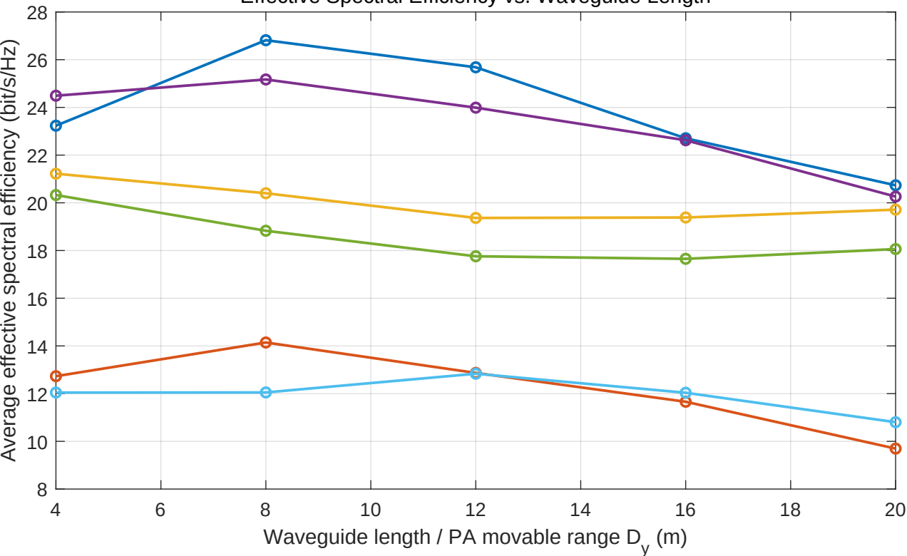
Effective Spectral Efficiency vs. Waveguide Length
