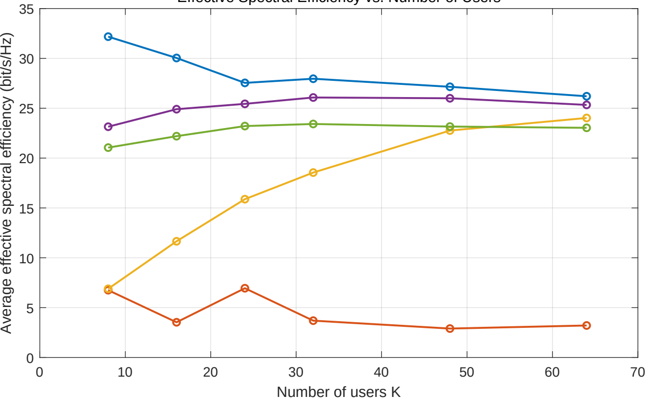
Effective Spectral Efficiency vs. Number of Users
