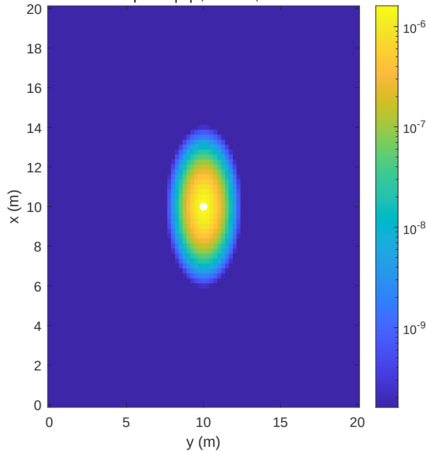
z = 0 plane |H|^2 , a=0.50 , b=0.30
