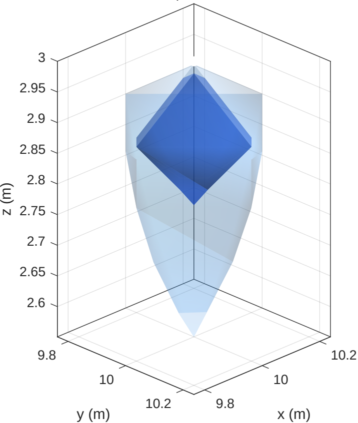
3D beam shape, a=0.50 , b=0.30
