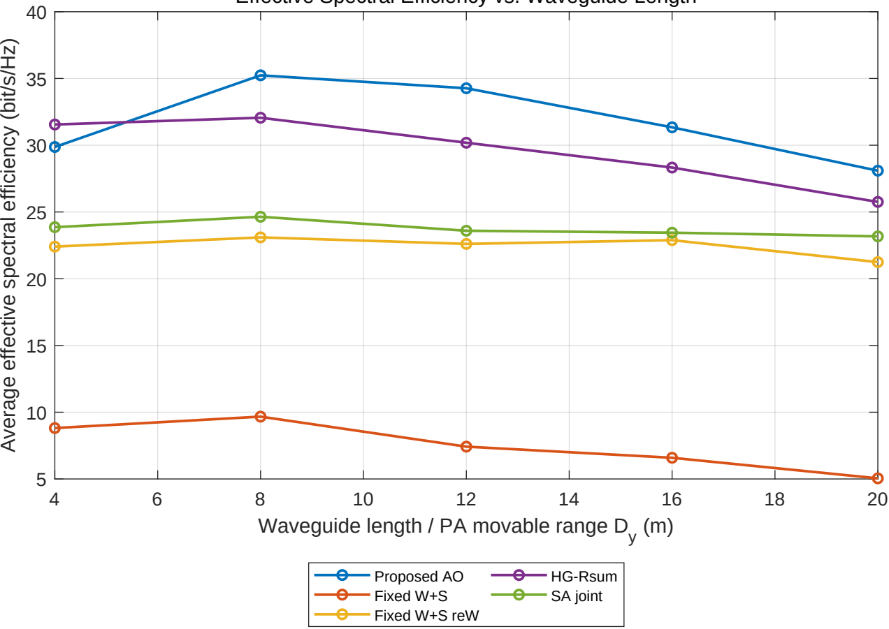
Effective Spectral Efficiency vs. Waveguide Length
