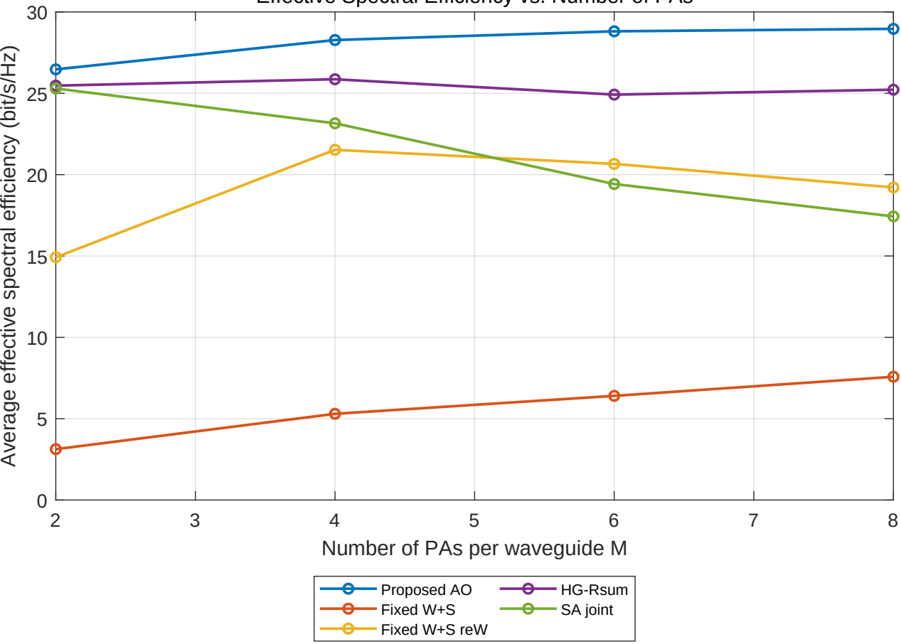
Effective Spectral Efficiency vs. Number of PAs
