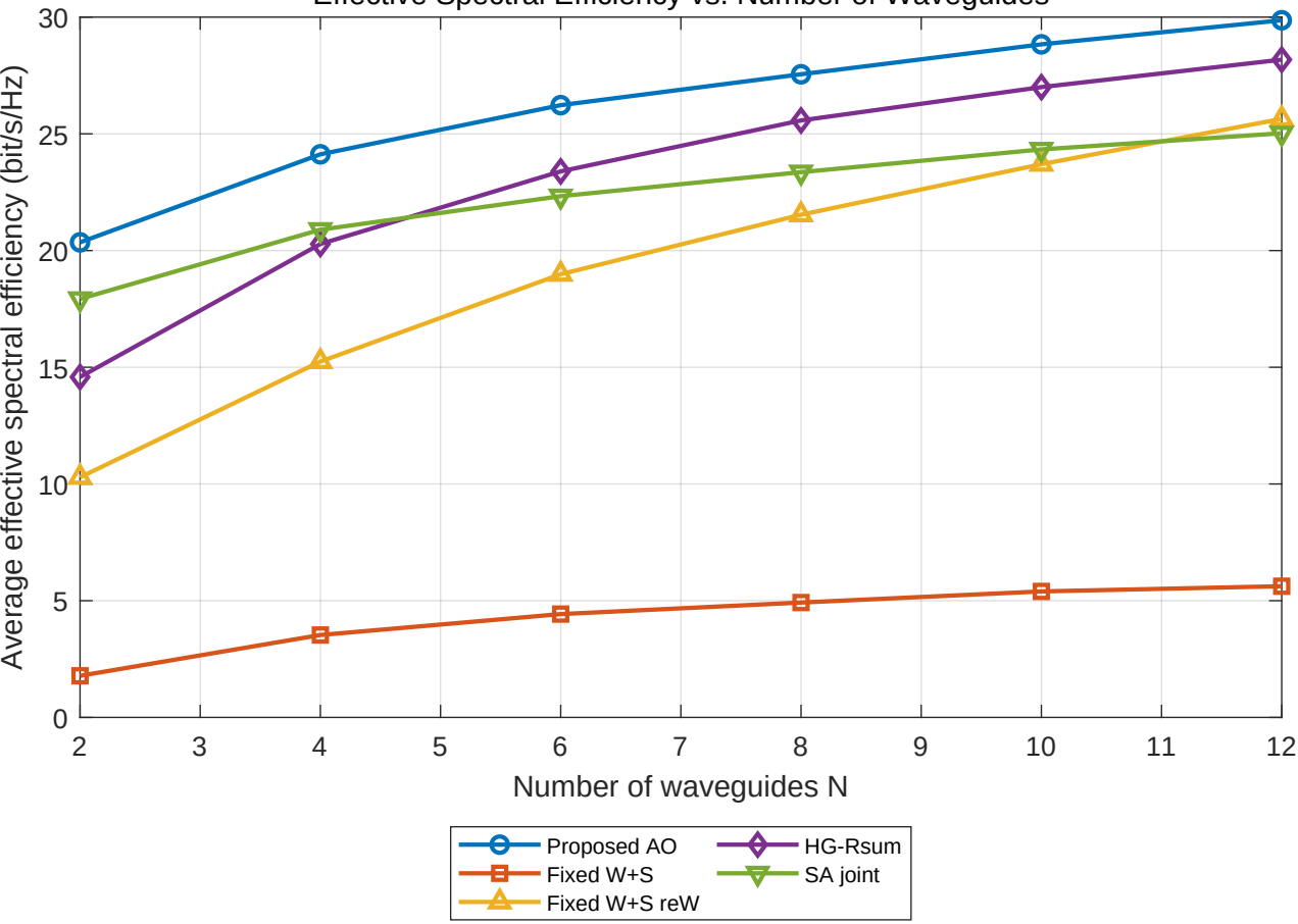
Effective Spectral Efficiency vs. Number of Waveguides
