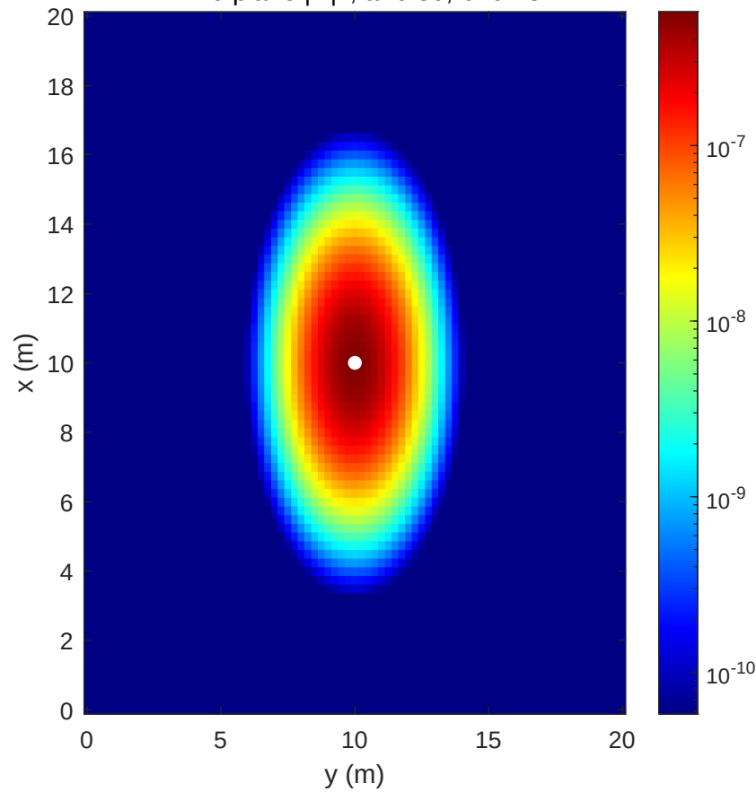
z = 0 plane |H|^2 , a=0.30 , b=0.18
