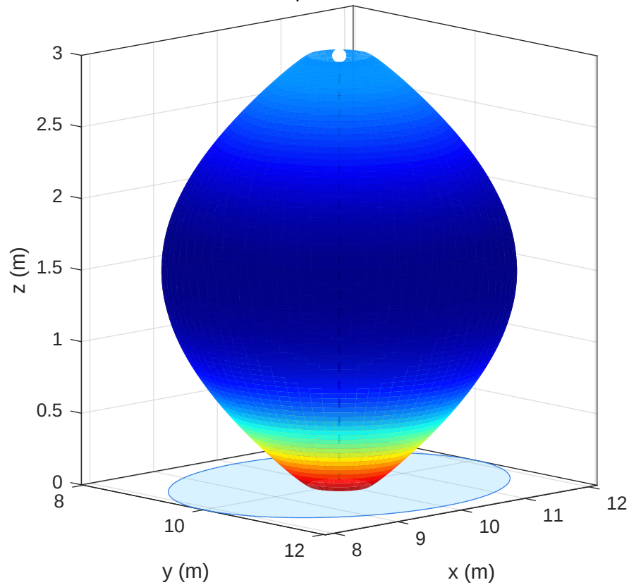
3D main lobe pattern, a=0.30 , b=0.18
