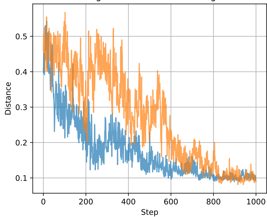
Average minimum distance to goal
