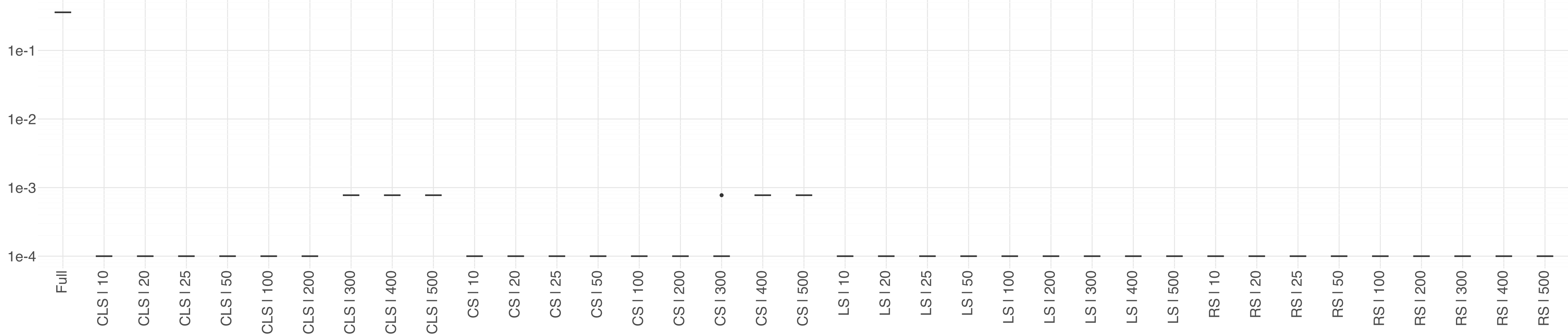
Method | k
