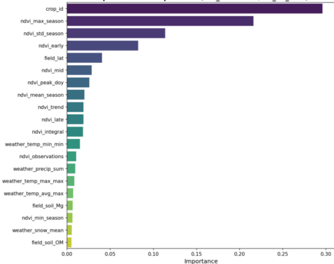
Top 20 Feature Importance (full_extended / all_no_leak)
