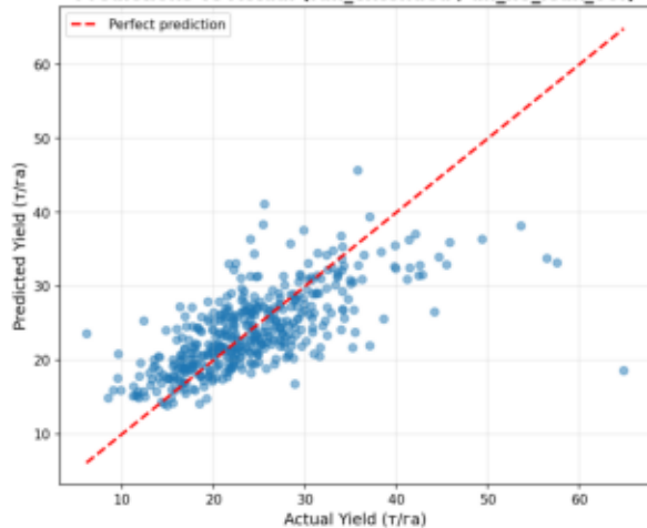
Predictions vs Actual (full_extended / all_no_leak_oof)
