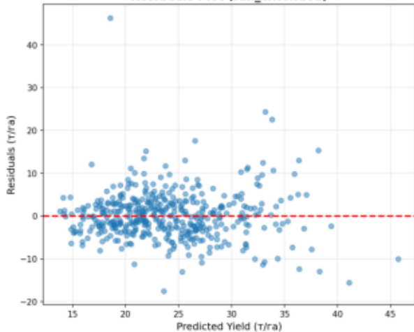
Residuals Plot (full_extended)
