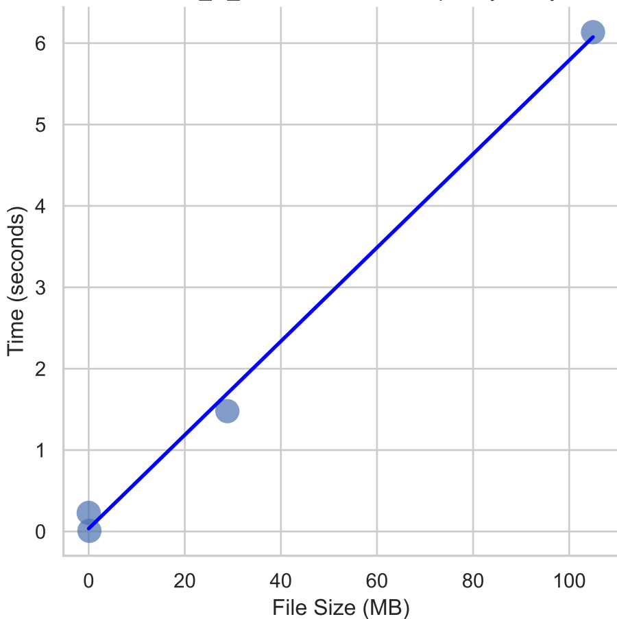
ORIGINAL_D_MOD - Decode Complexity Analysis
