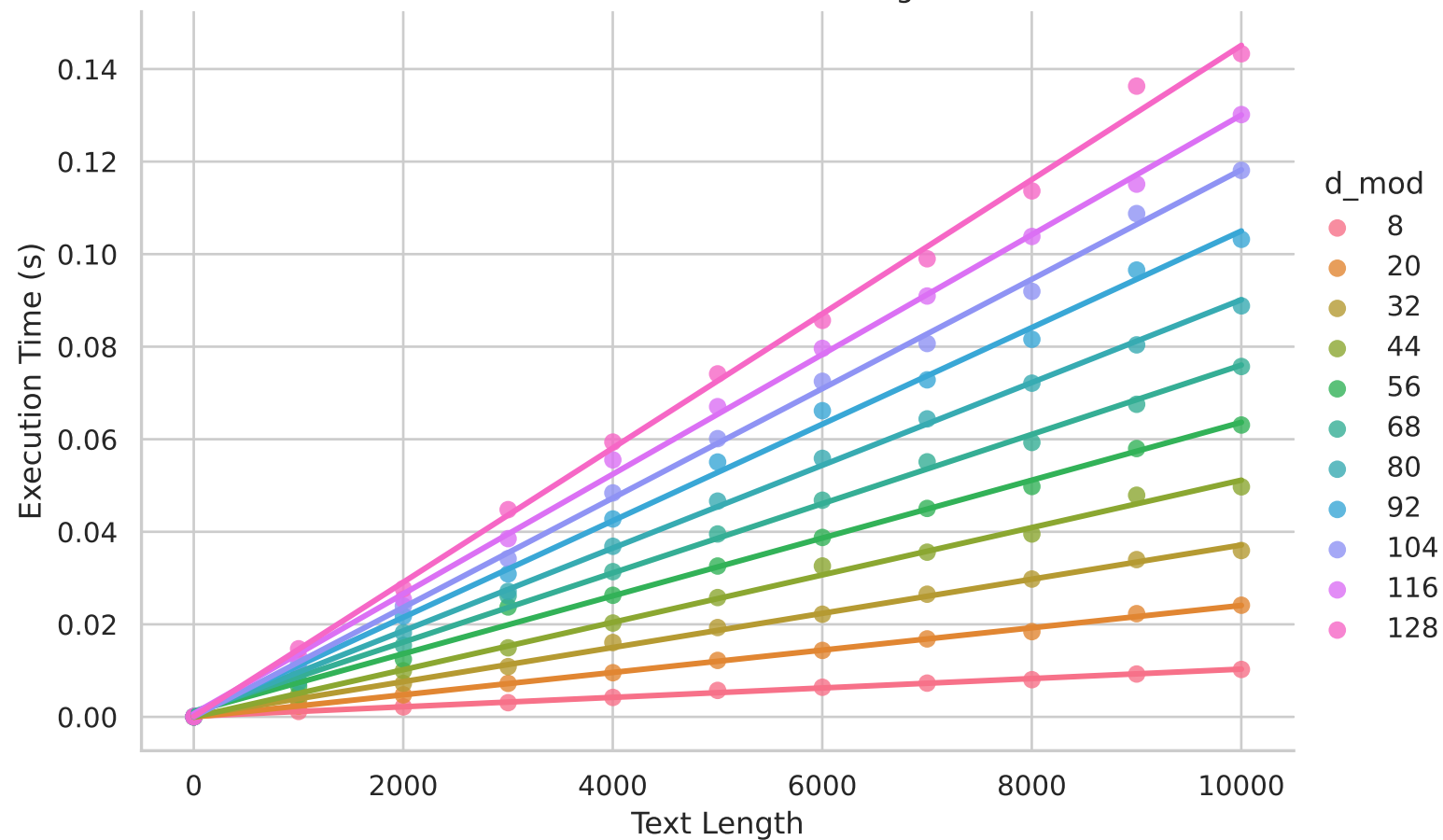
Execution Time vs Text Length
