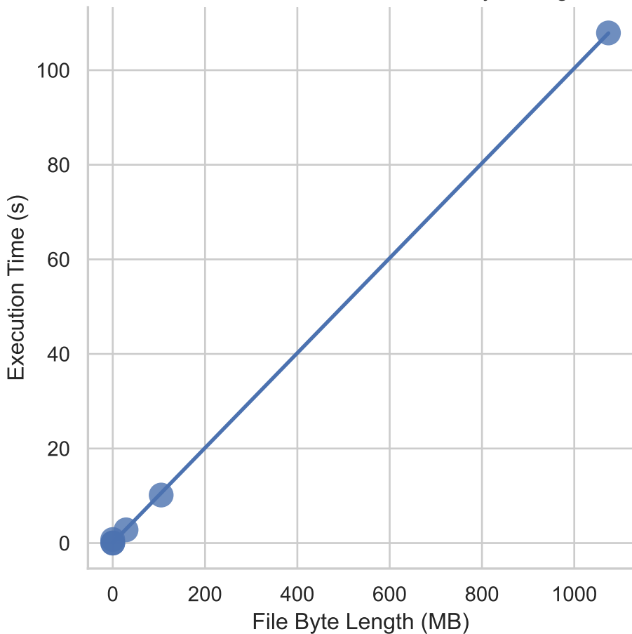
ENCODE Execution Time vs File Byte Length
