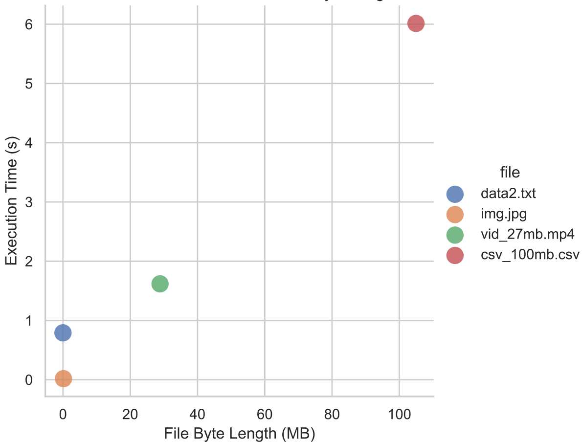
DECODE Execution Time vs File Byte Length
