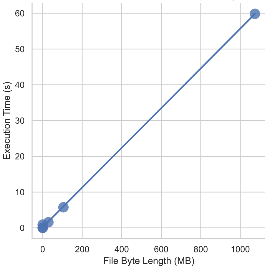
DECODE Execution Time vs File Byte Length
