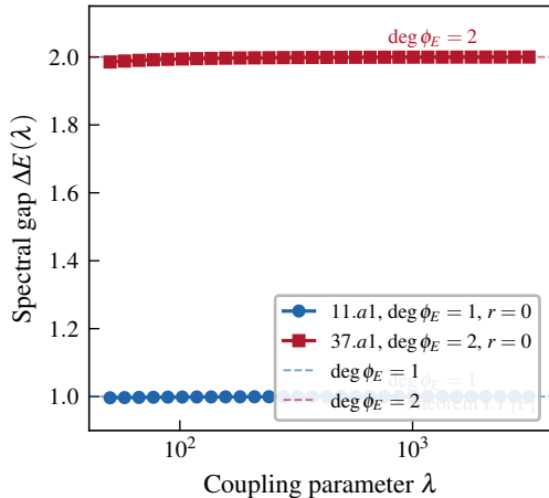
(a) Rank 0: \lim_{\lambda \rightarrow \infty} \Delta E(\lambda) = \deg \phi_E
