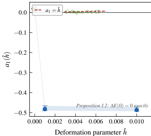
(b) Zoom: collapse at \hat{h} \rightarrow 0
