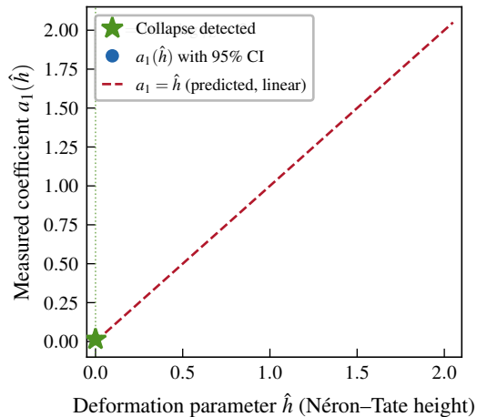
(a) Full range: \Delta E_y(\hat{h}) = \hat{h} + O(\hat{h}^2)
