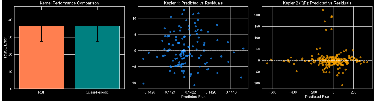
Figure 7: Comparative diagnostics for RBF and quasi-periodic kernel performance on the rotating-star dataset (KIC 007609553). The RMSE and MAE distributions across 20 Monte Carlo splits are near-indistinguishable between kernel classes, with substantial distributional overlap. The absence of a statistically meaningful improvement from the more expressive QP kernel is consistent with the hypothesis that globally stationary covariance assumptions represent the binding modeling constraint, rather than the particular form of the periodic component.
