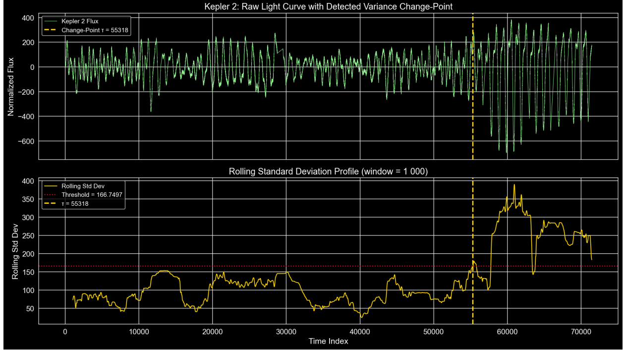
Figure 8: Detection of a variance regime shift in the Kepler 2 rotating-star light curve using rolling variance diagnostics. Top panel: The observed Kepler 2 flux time series with the detected change-point \tau indicated by the dashed vertical line. A substantial increase in oscillation amplitude is visible in the later portion of the light curve. Bottom panel: Rolling standard deviation profile computed with a sliding window of 1000 observations. The horizontal dotted line denotes the variance-shift threshold used for automatic change-point detection, while the vertical dashed line marks the inferred transition epoch. The results suggest the presence of evolving variability amplitude and motivate investigation of piecewise-stationary Gaussian Process models.
