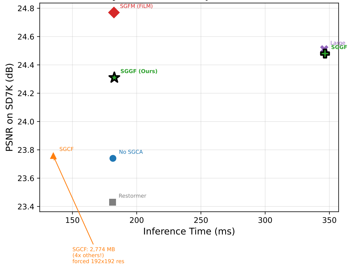
(b) Accuracy vs. Inference Speed (SD7K, 256x256)
