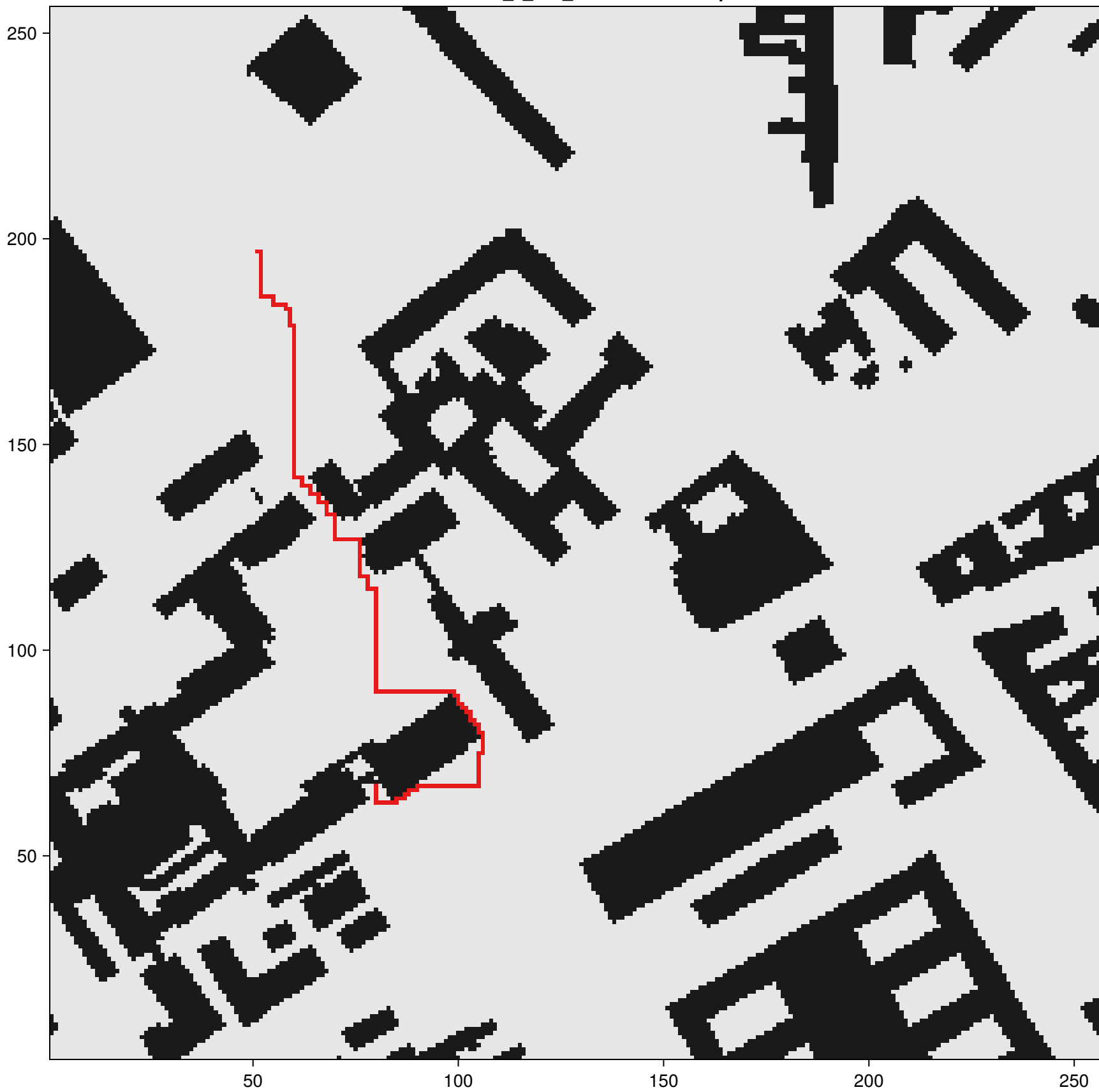
res/Berlin_0_256_solutionAstar.map
