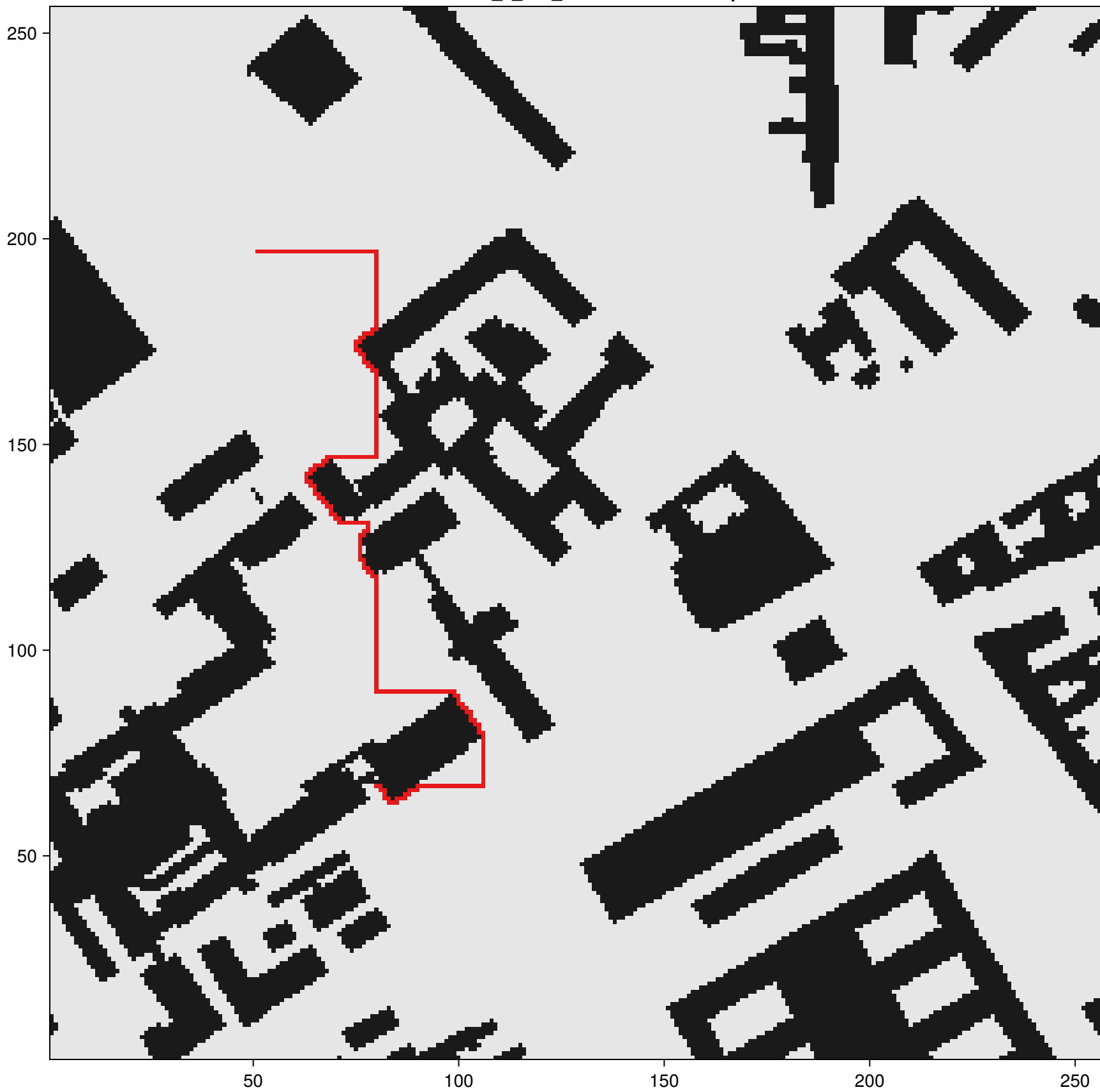
res/Berlin_0_256_solutionGlouton.map
