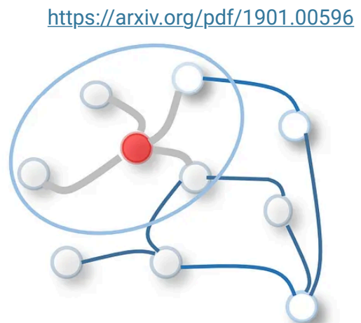
Figure 5: Principle of the graph diff pooling
