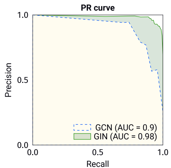
Figure 14: Precision-Recall curve comparing GCN and GIN approaches
