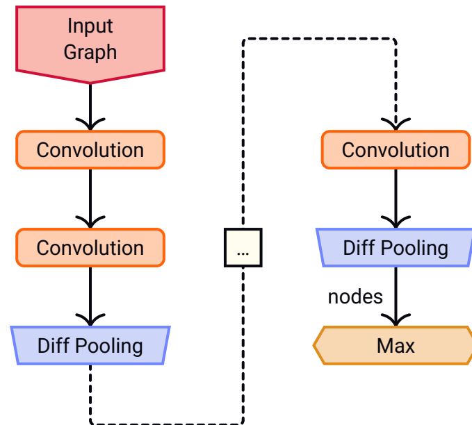
Figure 2: Graph compression process
