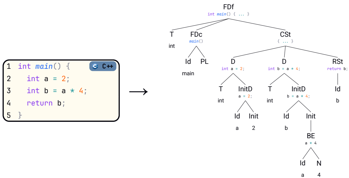
Figure 3: AST representation of a simple C++ program
