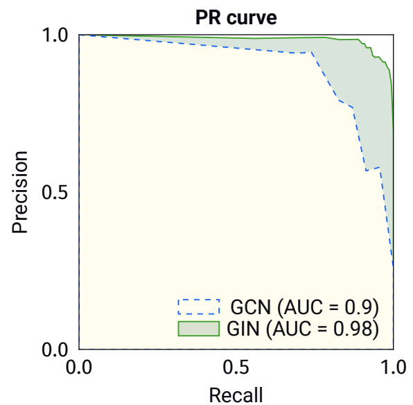
Figure 14: Precision-Recall curve comparing GCN and GIN approaches
