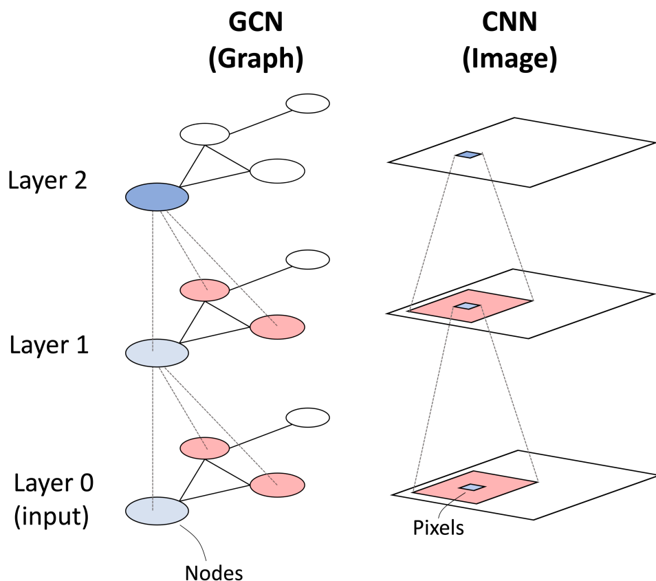
Figure 4: Principle of the graph convolution layer
