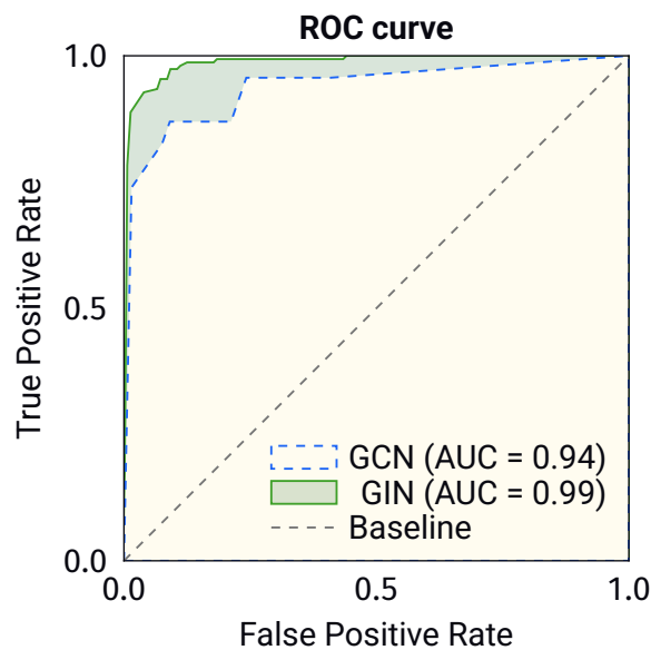
Figure 13: ROC curve comparing GCN and GIN approaches
