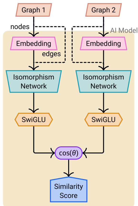
Figure 10: High-level ML pipeline for the GIN approach
