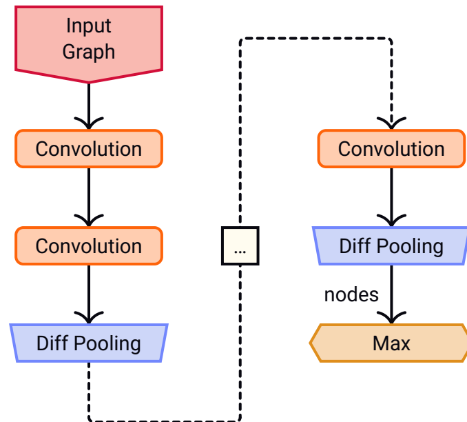
Figure 2: Graph compression process
