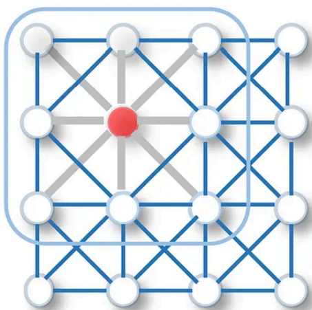
Figure 5: Principle of the graph diff pooling
