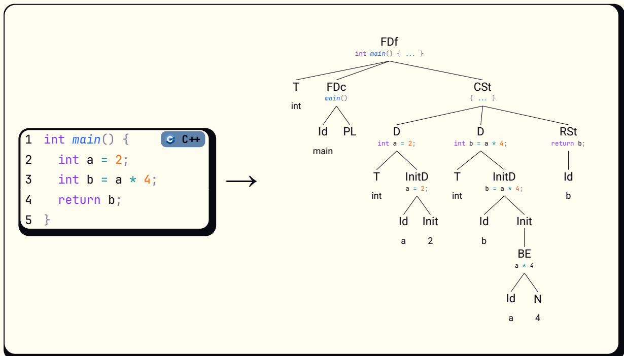
Figure 3: AST representation of a simple C++ program
