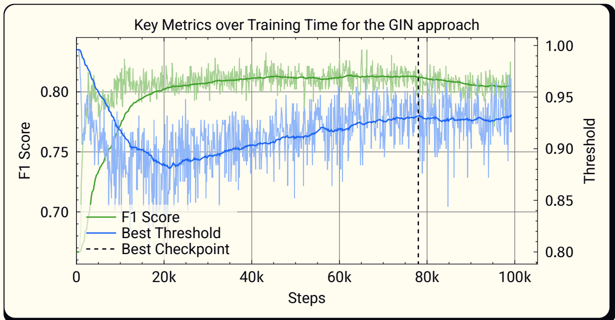
Figure 12: F1 Score and Best Threshold over Training Time for the GIN approach
