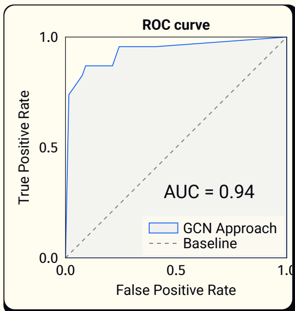
Figure 7: ROC curve for the GCN approach
