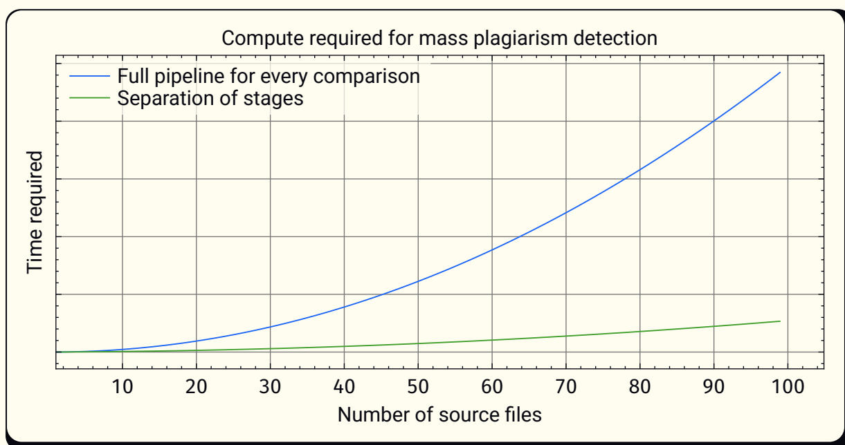
Figure 16: Time behavior comparison between full pipeline and stage separation
