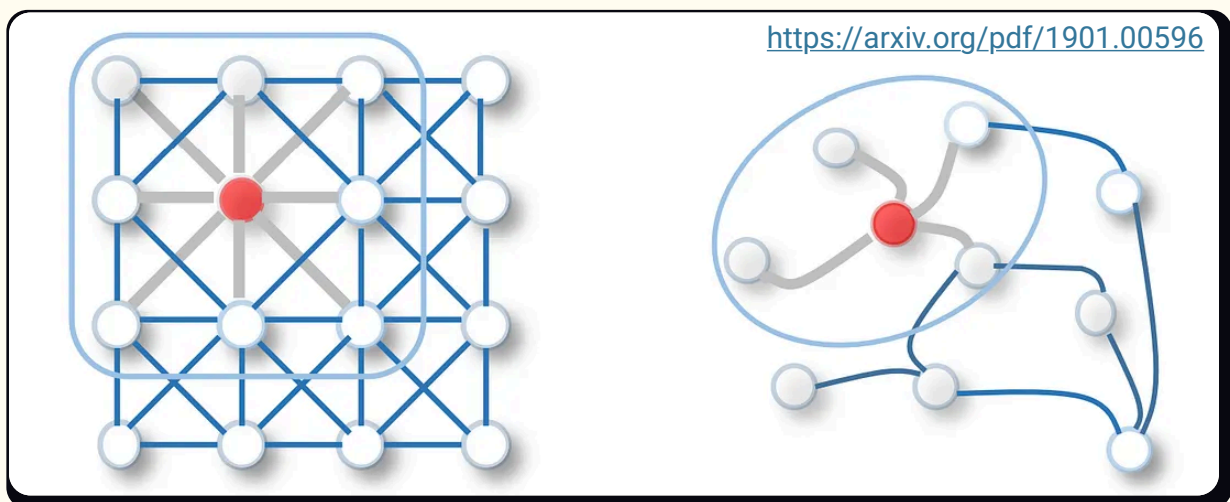
Figure 5: Principle of the graph diff pooling
