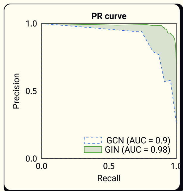
Figure 14: Precision-Recall curve comparing GCN and GIN approaches
