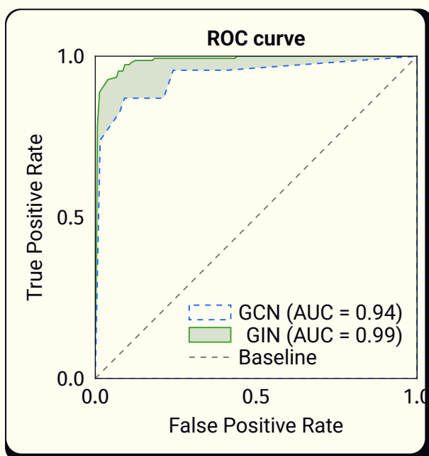
Figure 13: ROC curve comparing GCN and GIN approaches
