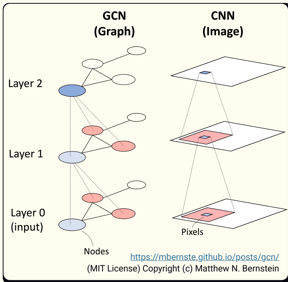
Figure 4: Principle of the graph convolution layer
