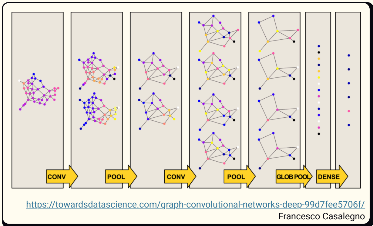
Figure 6: Stepwise graph feature condensation used for inspiration
