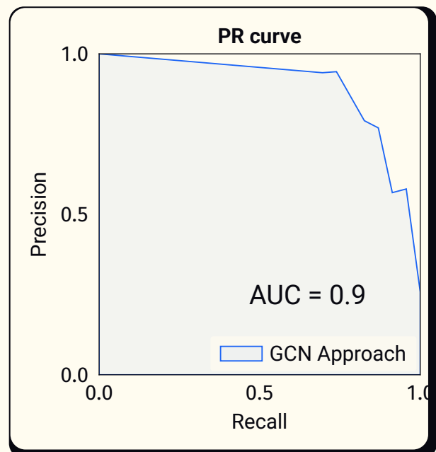
Figure 8: Precision-Recall curve for the GCN approach
