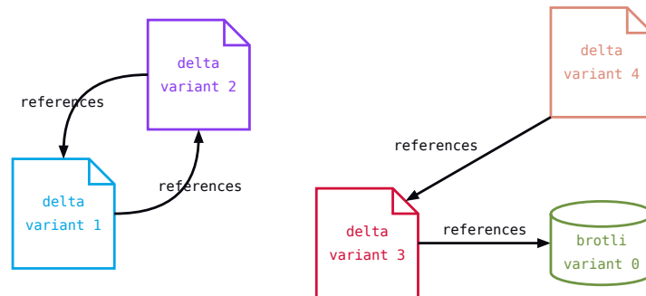
Listing 3: Cyclic delta compression references: Files represent delta patches, cylinders represent only brotli compressed full variants.
