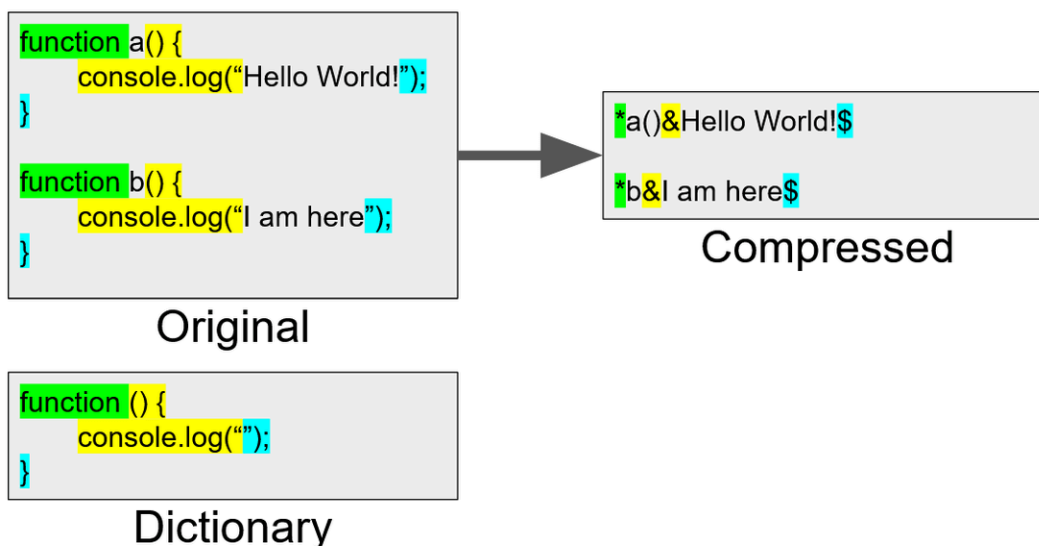
Figure 3: Dictionary compression in Brotli [Anna Monus, https://www.debugbear.com/blog/shared-compression-dictionaries ]
