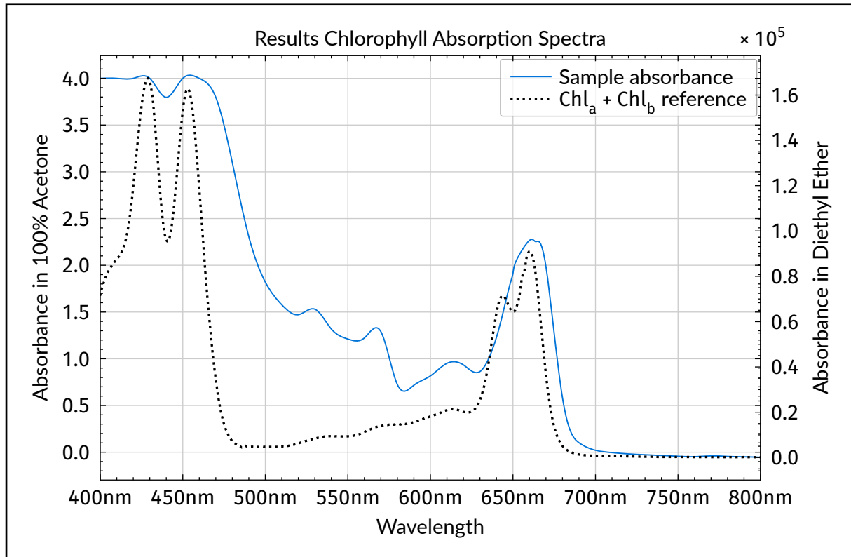
Figure 4: Absorption Spectrum of the Sample (shown in blue) and combined Chl a + Chl b Reference from Figure 3 (shown in dotted black)
