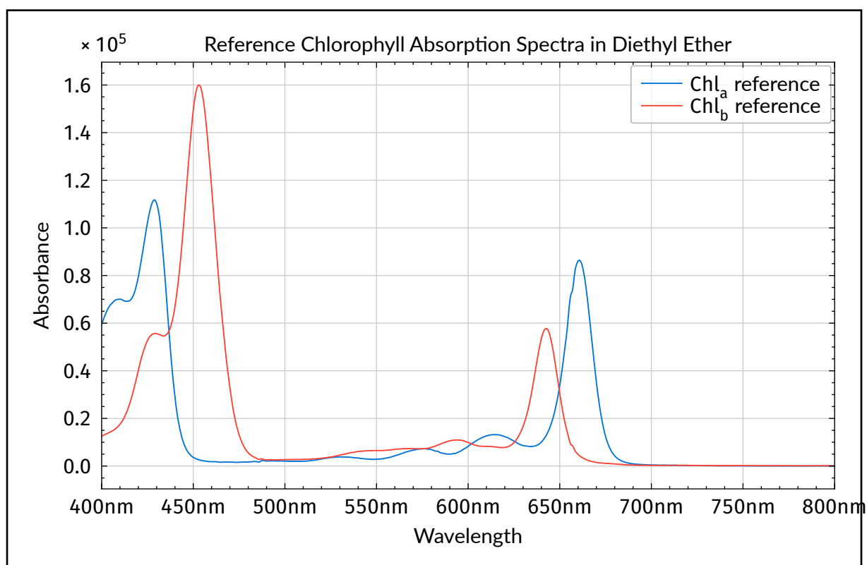
Figure 3: Reference Chlorophyll Absorption Spectra in Diethyl Ether [1], [2]
