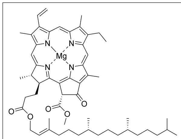
Figure 1: Chlorophyll A structure [1]
