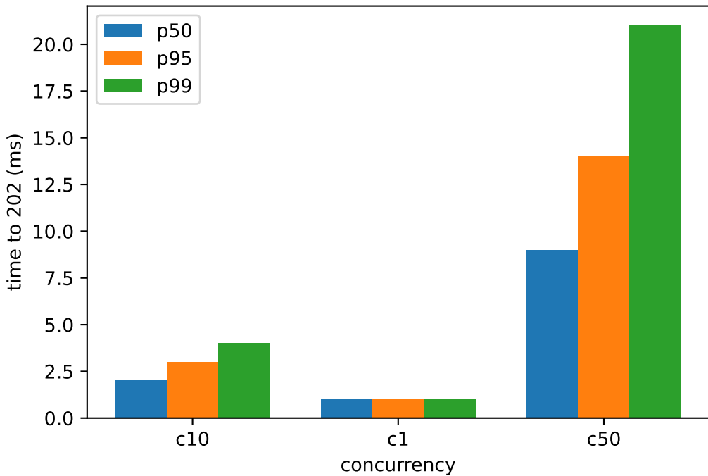
(a) POST /api/v1/segment/{type} 202 latency
