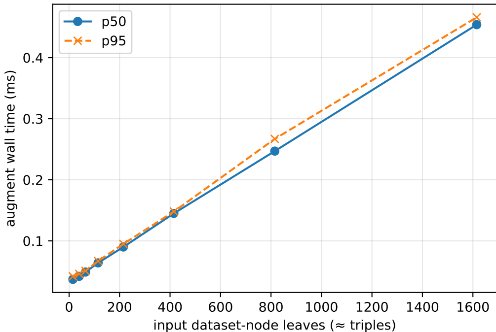
(b) Augmentation cost vs input size
