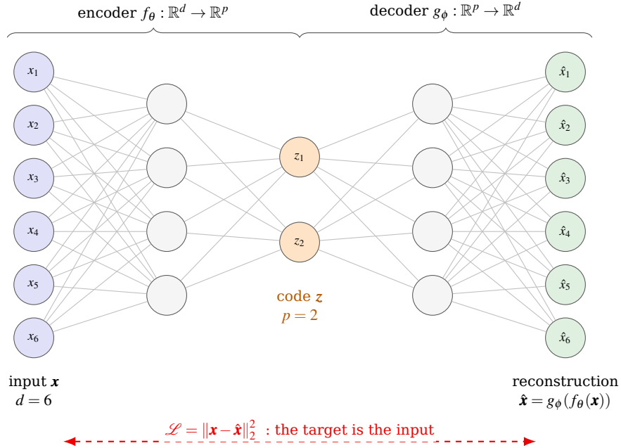
Fig. 12.1 An undercomplete autoencoder in the layer notation of Section 8.5, with d = 6 and p = 2 . Read left to right it is an ordinary feed-forward network of Figure 8.5; what makes it an autoencoder is the dashed arrow at the bottom, which says that the target of example n is example n itself. No labels enter anywhere, which is the content of the word self-supervised . Everything the network knows about \mathbf{x} after the encoder must pass through the two orange units, and the reconstruction is built from those two numbers alone.
