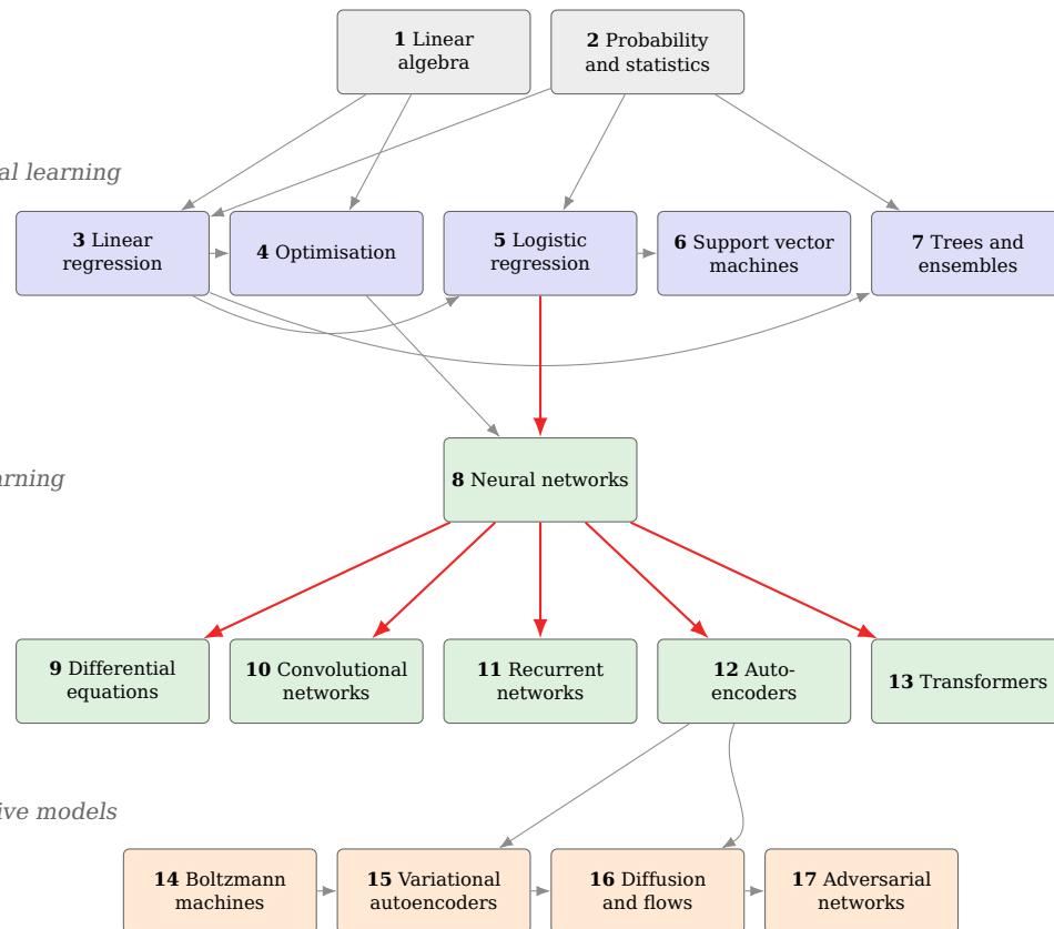
Fig. 18.1 The book as a graph. An arrow means that the later chapter uses a result of the earlier one, not merely that it comes after it. The two red paths are the ones the book is built around: logistic regression is a network with no hidden layer, so Chapter 8 begins by inserting one; and Chapters 9 to 13 all use the backpropagation of Section 8.8 unchanged – Chapters 10 to 13 by changing what structure is imposed on the weight matrix, Chapter 9 by keeping the network and changing the question it is asked. Two links are not drawn because they would cross the whole figure. The linear autoencoder of Chapter 12 rediscovers the singular value decomposition of Chapter 1 – that is Theorem 12.5 – and the Boltzmann machine of Chapter 14 is sampled by the Metropolis algorithm of Section 2.14.
