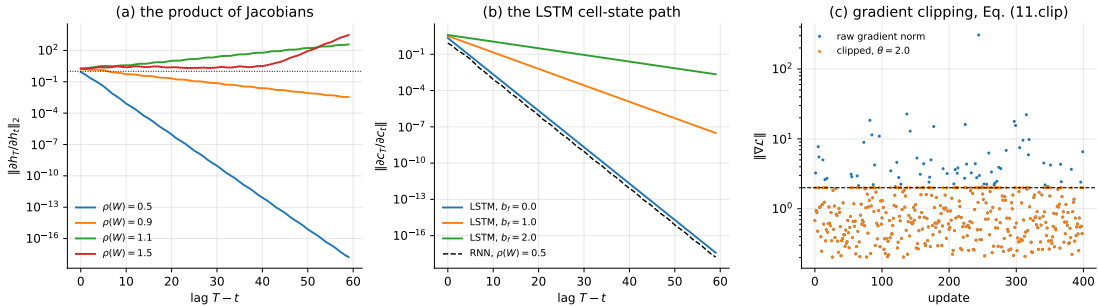
Fig. 11.2 (a) The spectral norm of the Jacobian product (11.19) against the lag T - t , for four values of the spectral radius of \mathbf{W} . The exponential behaviour of Theorem 11.1 is the straight line on a logarithmic axis. (b) The same quantity for the cell state of an LSTM, Eq. (11.29), at three values of the forget-gate bias, with the \rho = 0.5 curve of panel (a) repeated as a dashed line. At b_f = 0 the LSTM is no better than the vanilla RNN; the advantage comes entirely from biasing the gate open. (c) Gradient clipping, Eq. (11.23): the rare large norms that would otherwise destroy the parameters are rescaled, the direction is kept and everything below the threshold is untouched.
