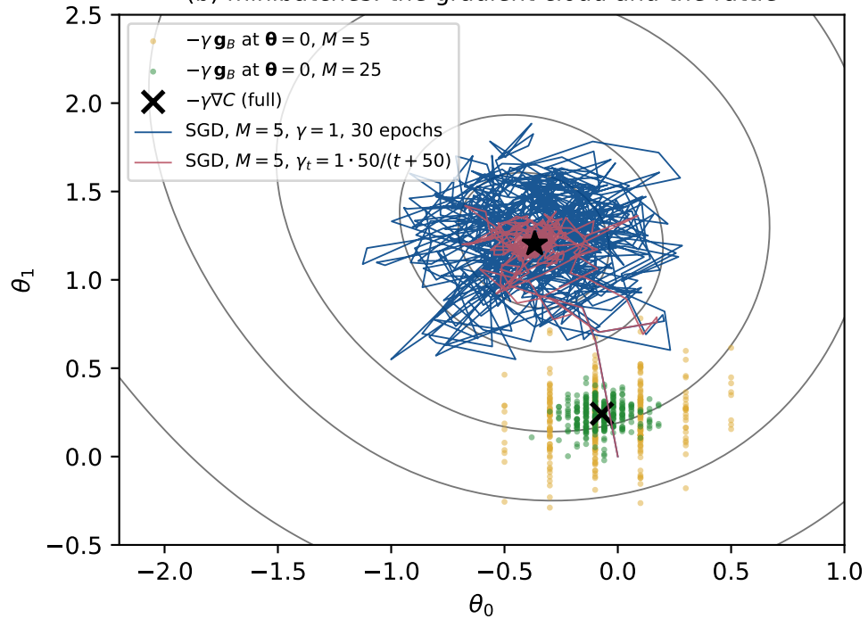
(b) minibatches: the gradient cloud and the rattle
