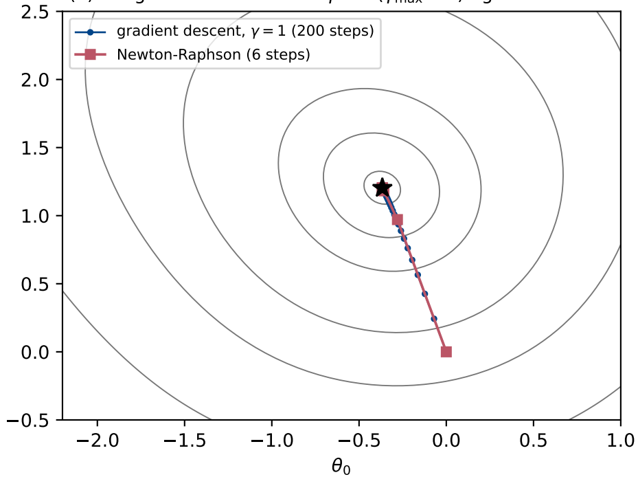
(a) full gradient: descent at \gamma = 1 ( \gamma_{\max} = 8 ) against Newton
